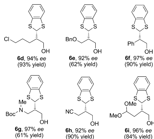
Scheme 2. Organocatalytic alkylation of functionalized aldehydes 4b–i with the cation 3a .
